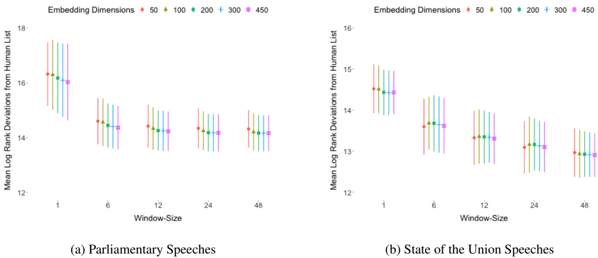
Figure 22: Human Preferences-Log Rank Deviations
